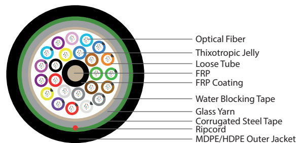
288 Fiber 24x12
