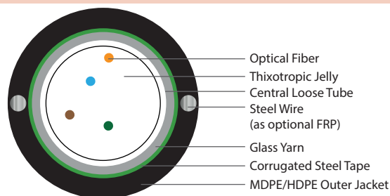
8 Fiber 1x8
