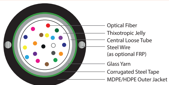
24 Fiber 1x24
