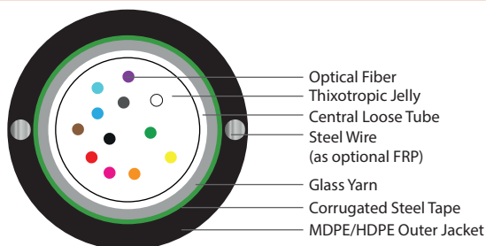
12 Fiber 1x12
