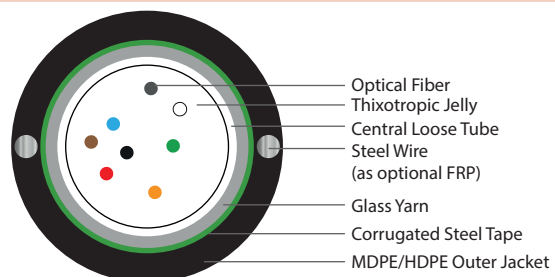
24 Fiber 1x24
