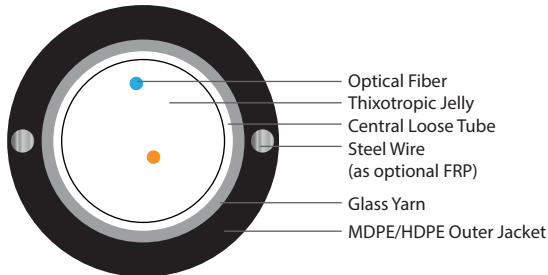
6 Fiber 1x6
