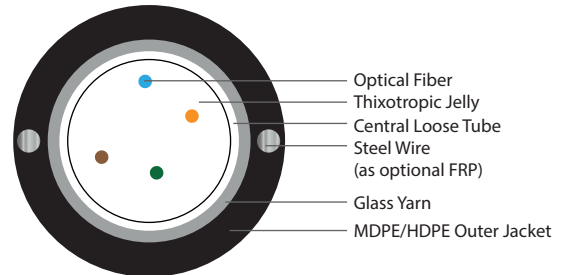
8 Fiber 1x8
