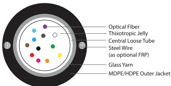
12 Fiber 1x12
