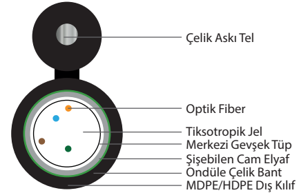
8 Fiber 1x8
