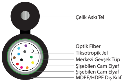
12 Fiber 1x12
