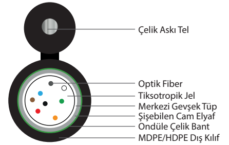
24 Fiber 1x24
