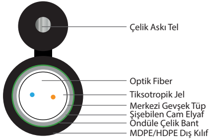
6 Fiber 1x6
