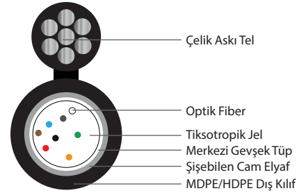
24 Fiber 1x24
