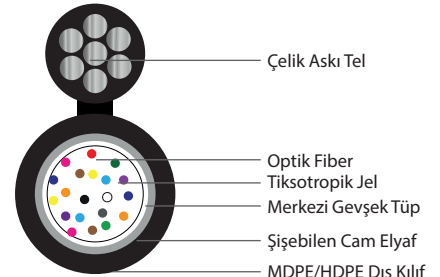
24 Fiber 1x24
