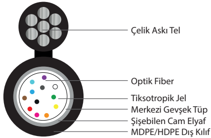
12 Fiber 1x12
