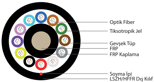
144 Fiber 12x12
