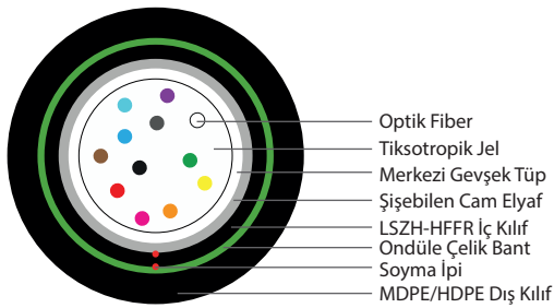
12 Fiber 1x12
