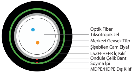
6 Fiber 1x6
