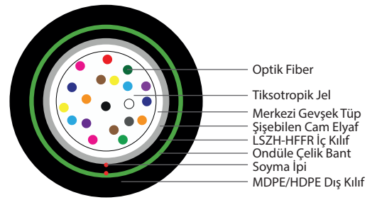
24 Fiber 1x24
