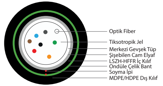
24 Fiber 1x24
